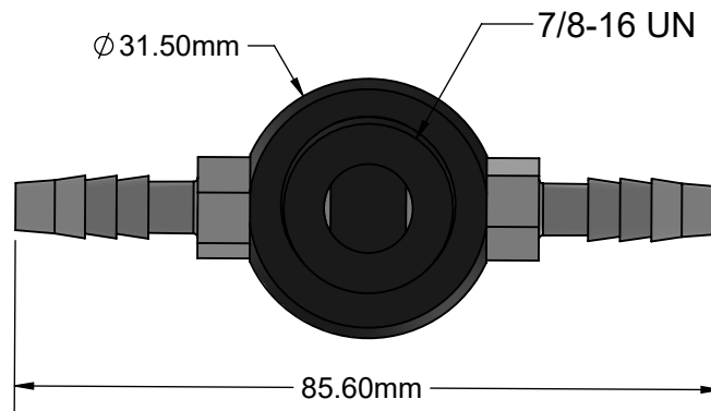
AO-002 Flow Through Head
