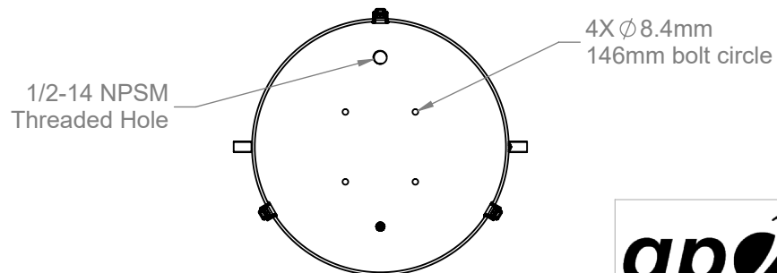
8 in diameter inlet (NWS)
