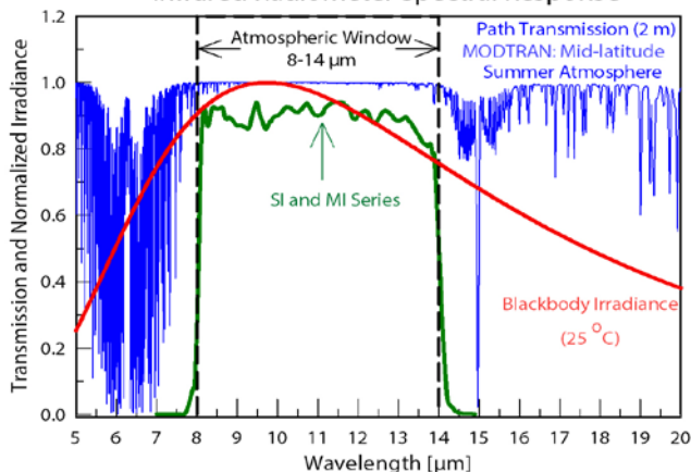
Infrared Radiometer Spectral Response
